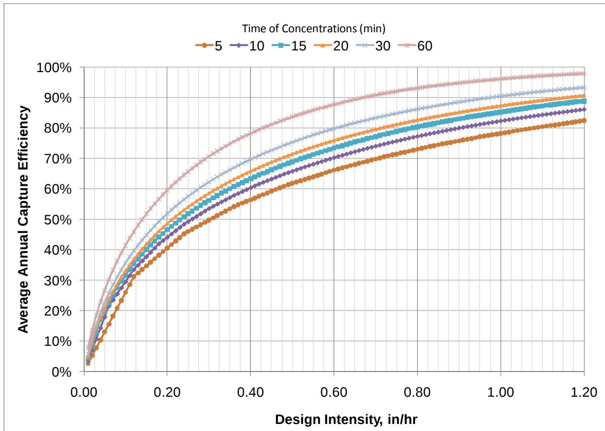
Figure 4-8: Percent Capture Nomograph for Flow-Based BMPs
